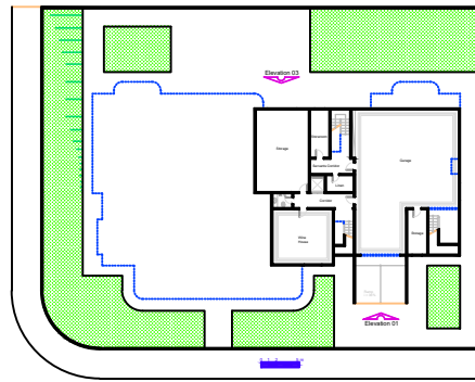
Lower Floor Plan A = 297,99 m 2
