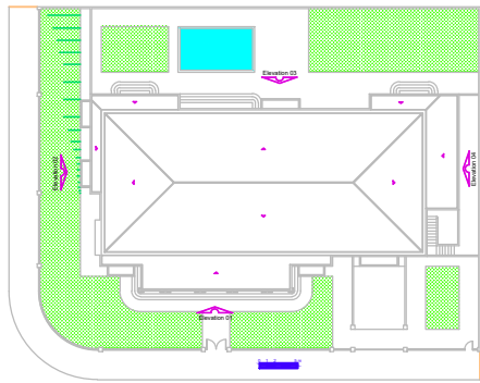
Roof Plan
