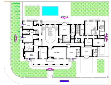
Second Floor Plan A = 567,38 m 2
